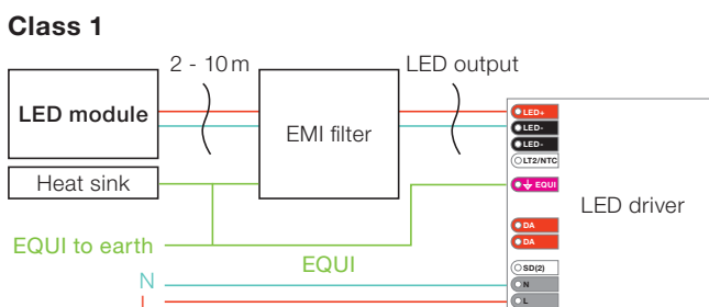
Figure 48: Connection for Class 1 configuration
