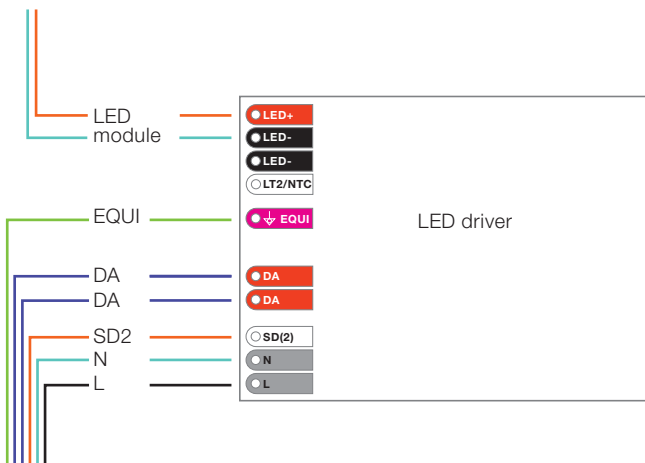
Figure 47: Recommended EMI wiring setup
