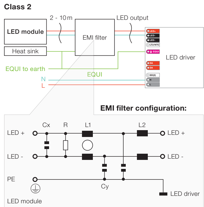
Figure 49: Connection for Class 2 with EQUI configuration
