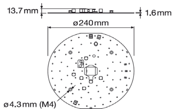
PL-FLAT-AC-MA-G3 2500-840 230V
