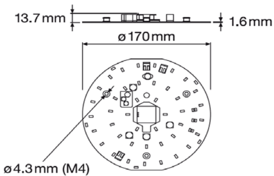
PL-FLAT-AC-MA-G3 1500-840 230V
