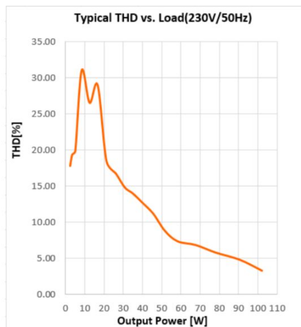
Typical THD vs Load-IT DALI 100 220-240 LT2 L
