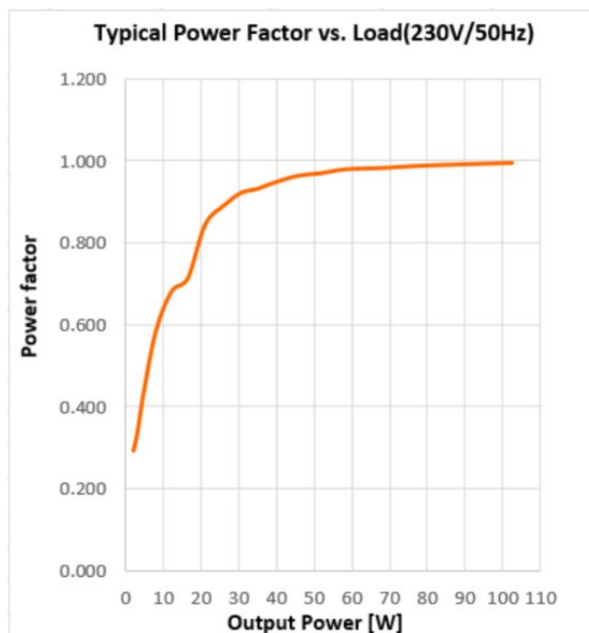
Typical Power Factor vs. Load-IT DALI 100 220-240 LT2 L
