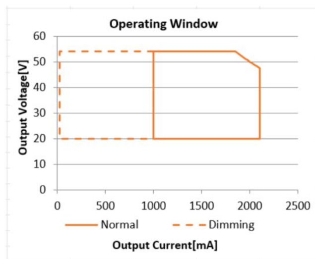
Operation Window-IT DALI 100 220-240 LT2 L
