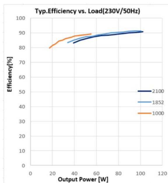
Typical Efficiency Vs. Load-IT DALI 100 220-240 LT2 L
