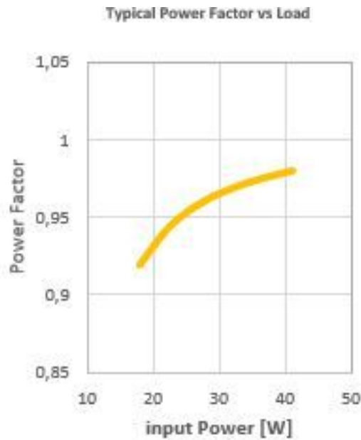
ETI DALI 35 LT2 L Typical Power Factor vs. Load
