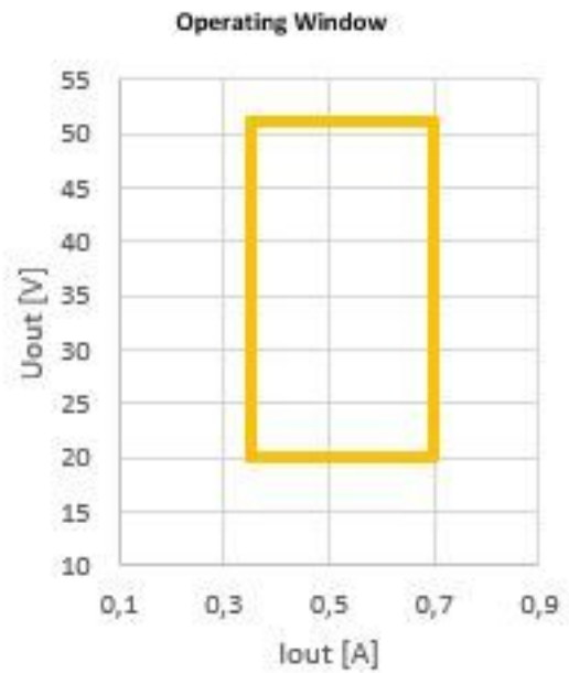
ETI DALI 35 LT2 L Operating Window
