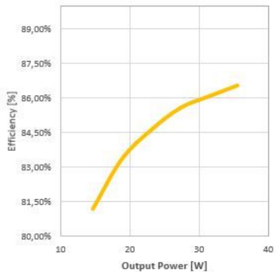
ETI DALI 35 LT2 L Typical Efficiency vs. Load
