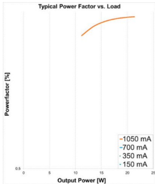
OTI DALI 15/220-240/1A0 NFC Typical Power Factor vs. Load
