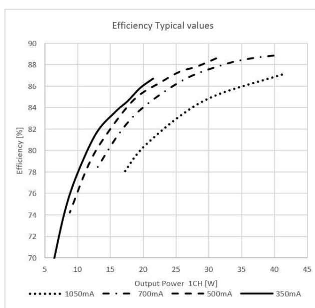
OT DX 40W 2C Typical Efficiency vs Load 230V 50Hz
