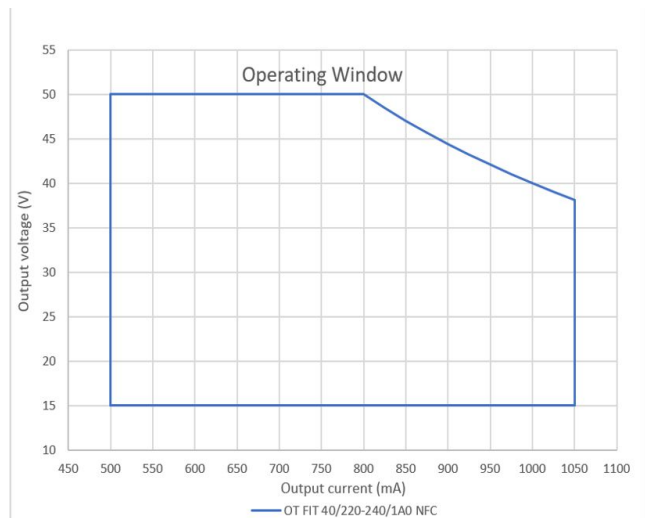
OT FIT 40 NFC G2 Operating window
