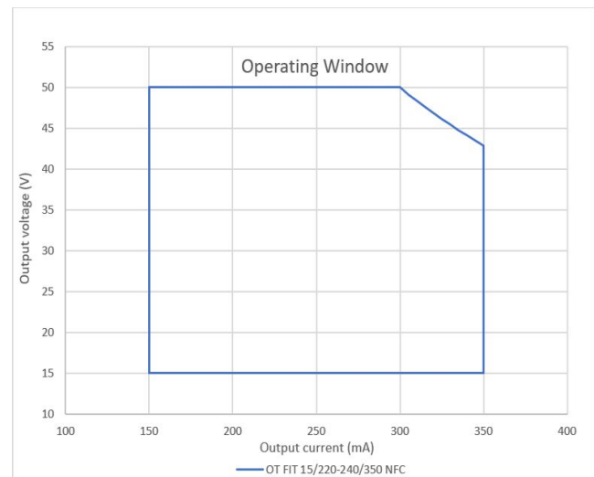
OT FIT 15 NFC G2 Operating window
