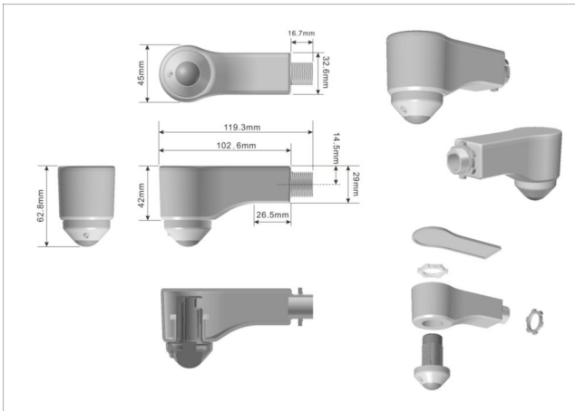
Batten mount adapter
